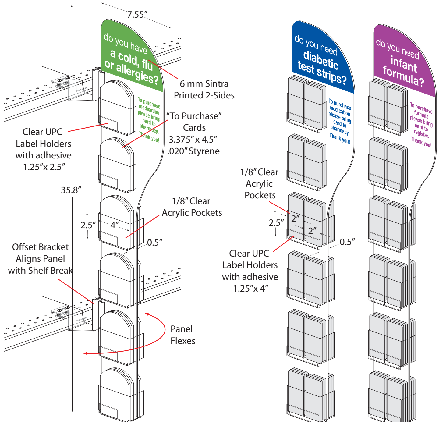
Standard Under Shelf Flex Bracket holds 1/8" to 1/4" material
